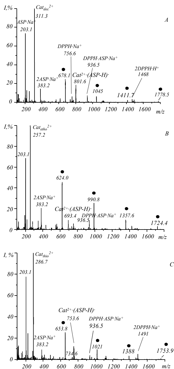
Fig. 3. ESI mass spectra of triple BQAC:ASP:DPPC systems: A – BQAC is decamethoxinum; B – BQAC is ethonium; C – BQAC is thionium. Sets of peaks corresponding to [\text{Cat} \cdot n\text{DPPC}]^+ complexes ( n = 1 \div 4 ) are marked by (•) symbol
